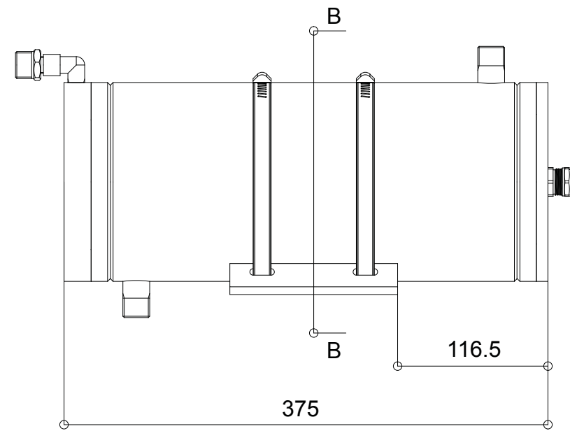
FIXING BASE
